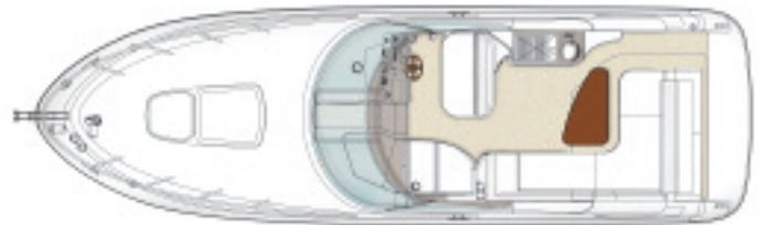
Cockpit Layout
