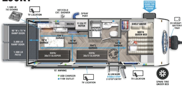
Length: 25' 0" • UVW: 4,488 lb.
