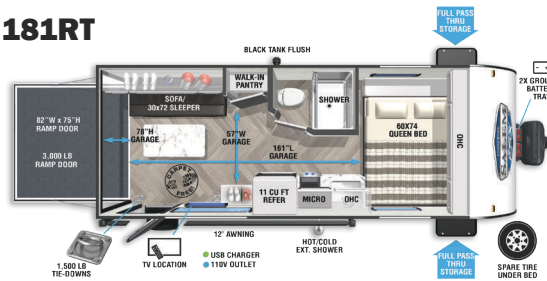
Length: 21' 8" • UVW: 3,204 lb.
