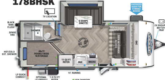
Length: 22' 11" • UVW: 3,749 lb.
