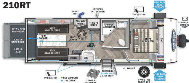
Length: 28' 8" • UVW: 4,997 lb.
