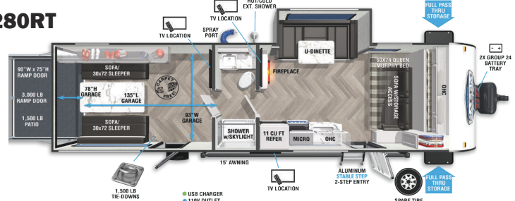
Length: 32' 4" • UVW: 5,608 lb.
